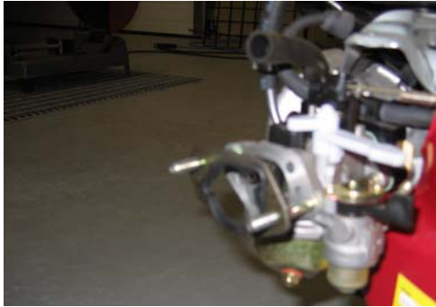
7) Locate carburetor and shroud gasket on carburetor mounting studs
