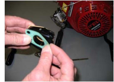
4) Carefully remove gaskets from insulator
